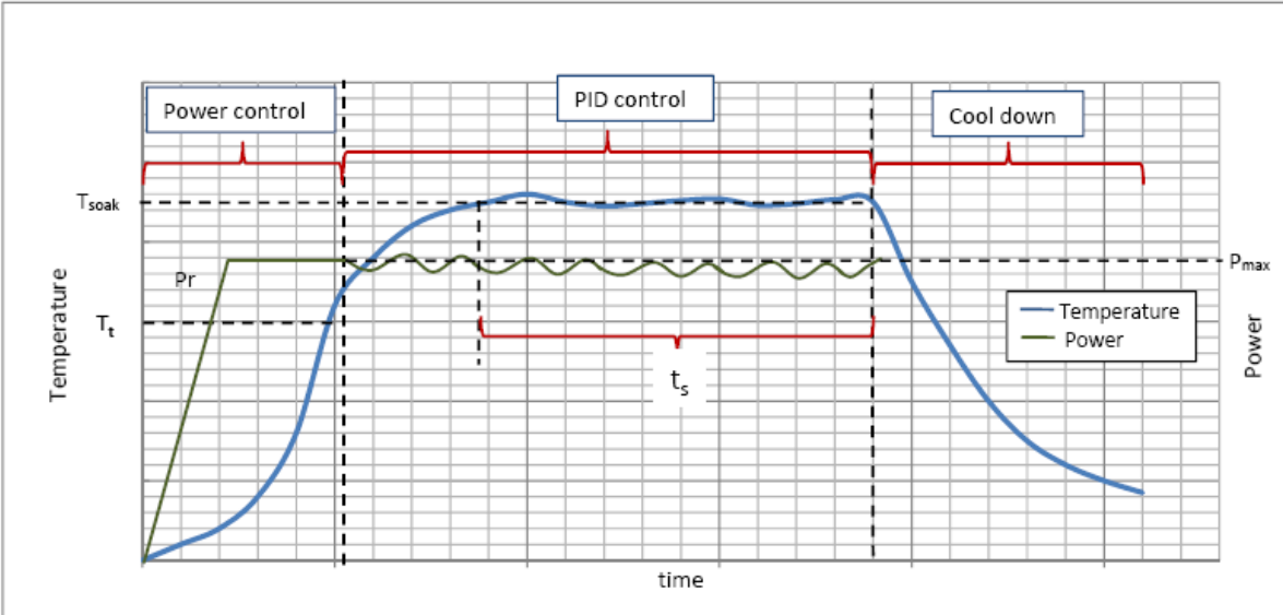
Figure 2 – Dual Mode Control Theory
